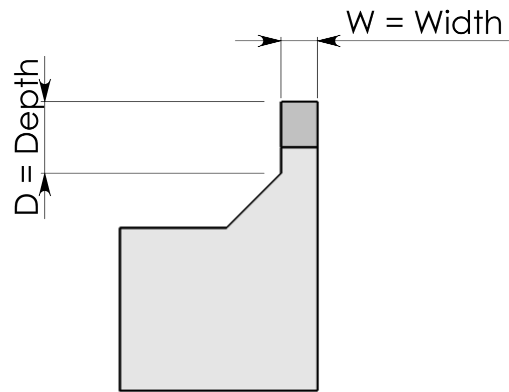
Standard Anvil W = 2.40mm D = 4.70mm
